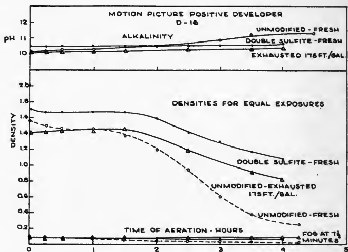
FIG. 1. Effect of prolonged aeration on an elon-hydroquinone developer (Formula D-16).
